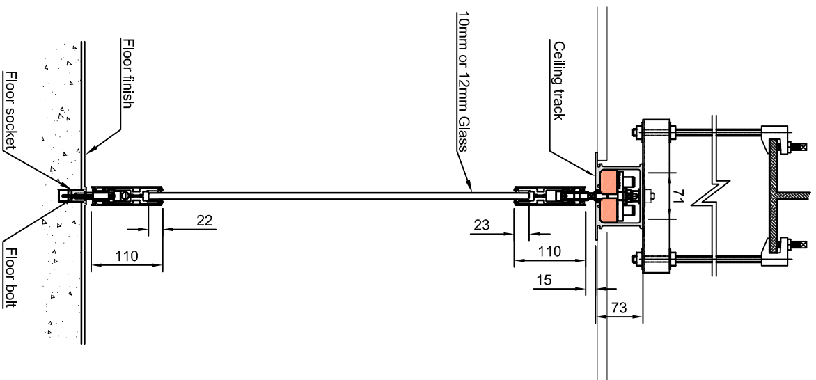
VERTICAL SECTION OF PANEL & TRACK FIXING
