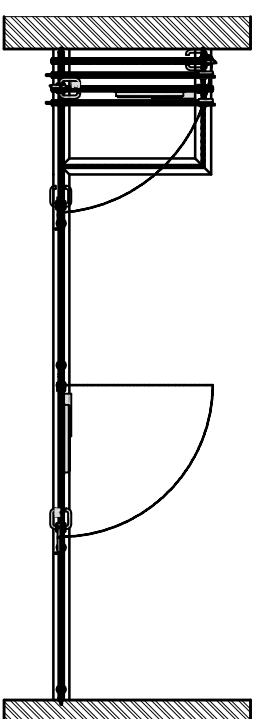
PLAN
